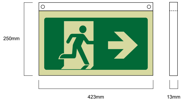
Diagram: Based on 24M Apollo Heavy Duty Exit Sign
