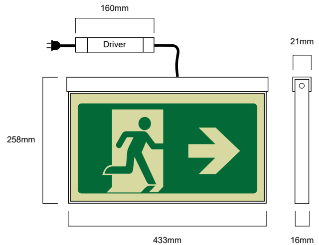
Diagram: Based on 24m Theia Hybrid Exit Sign
